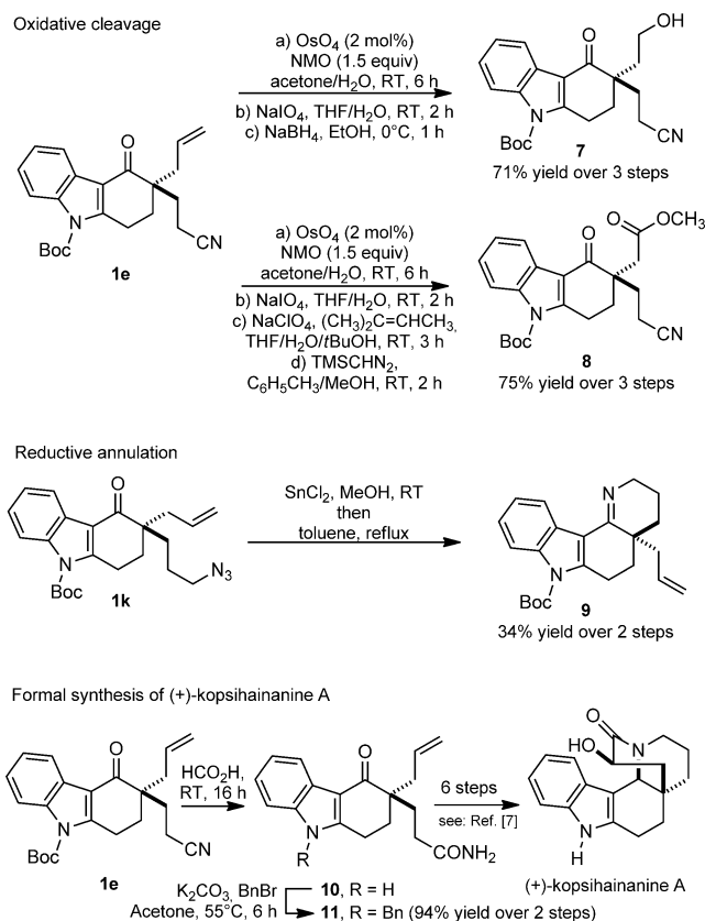
Scheme 3. Derivatization.
